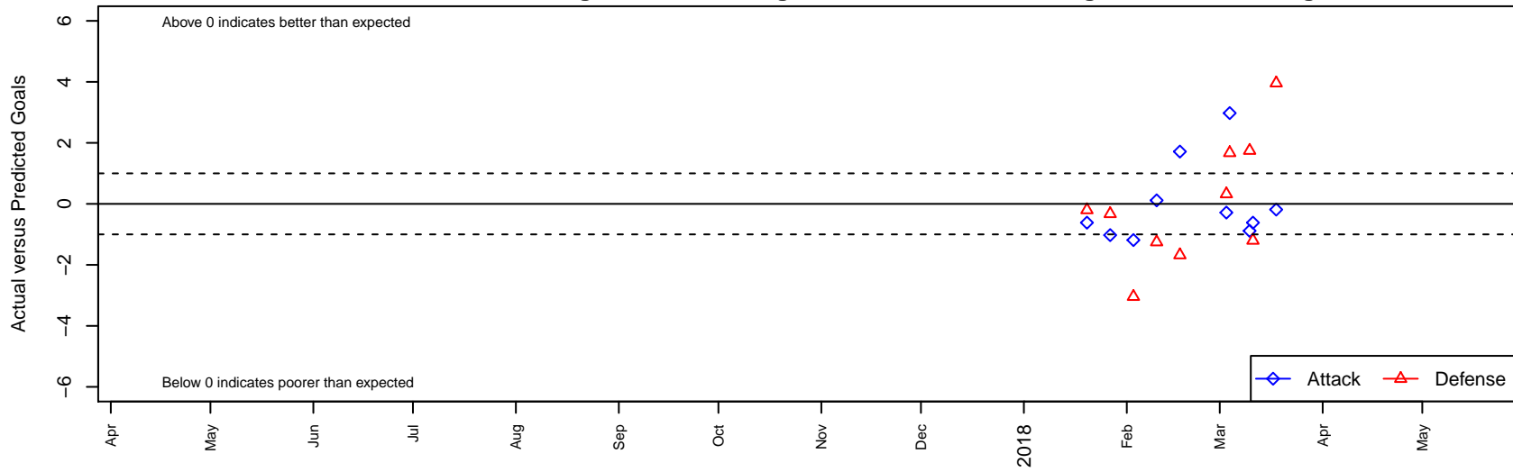
BSC Hood River Dynamos G99 Dots are actual minus expected GF (blue circles) and GA (red triangles). Blue line is smoothed change in attack strength. Red is smoothed change in defense strength.
